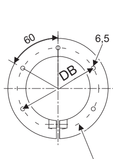
DB Bodenring DB floor flange
