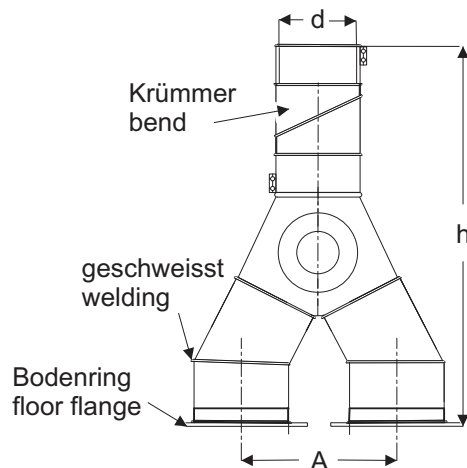
DB Bodenring DB floor flange
